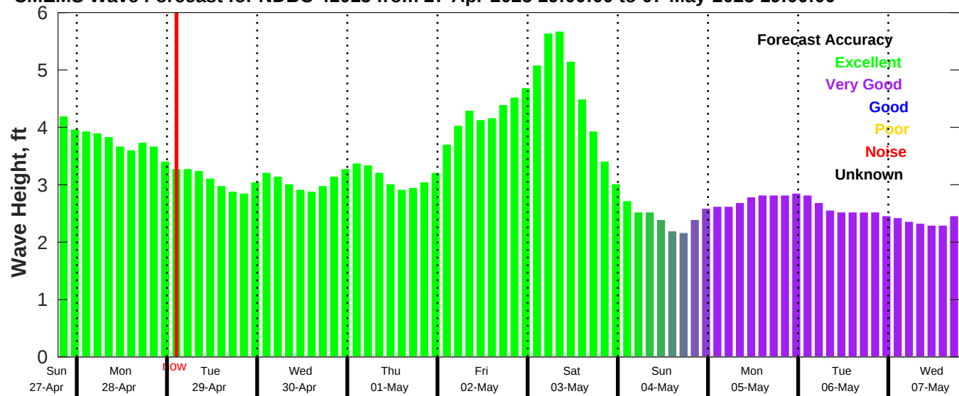
CMEMS Wave Forecast for NDBC 41013 from 27-Apr-2025 19:00:00 to 07-May-2025 19:00:00
