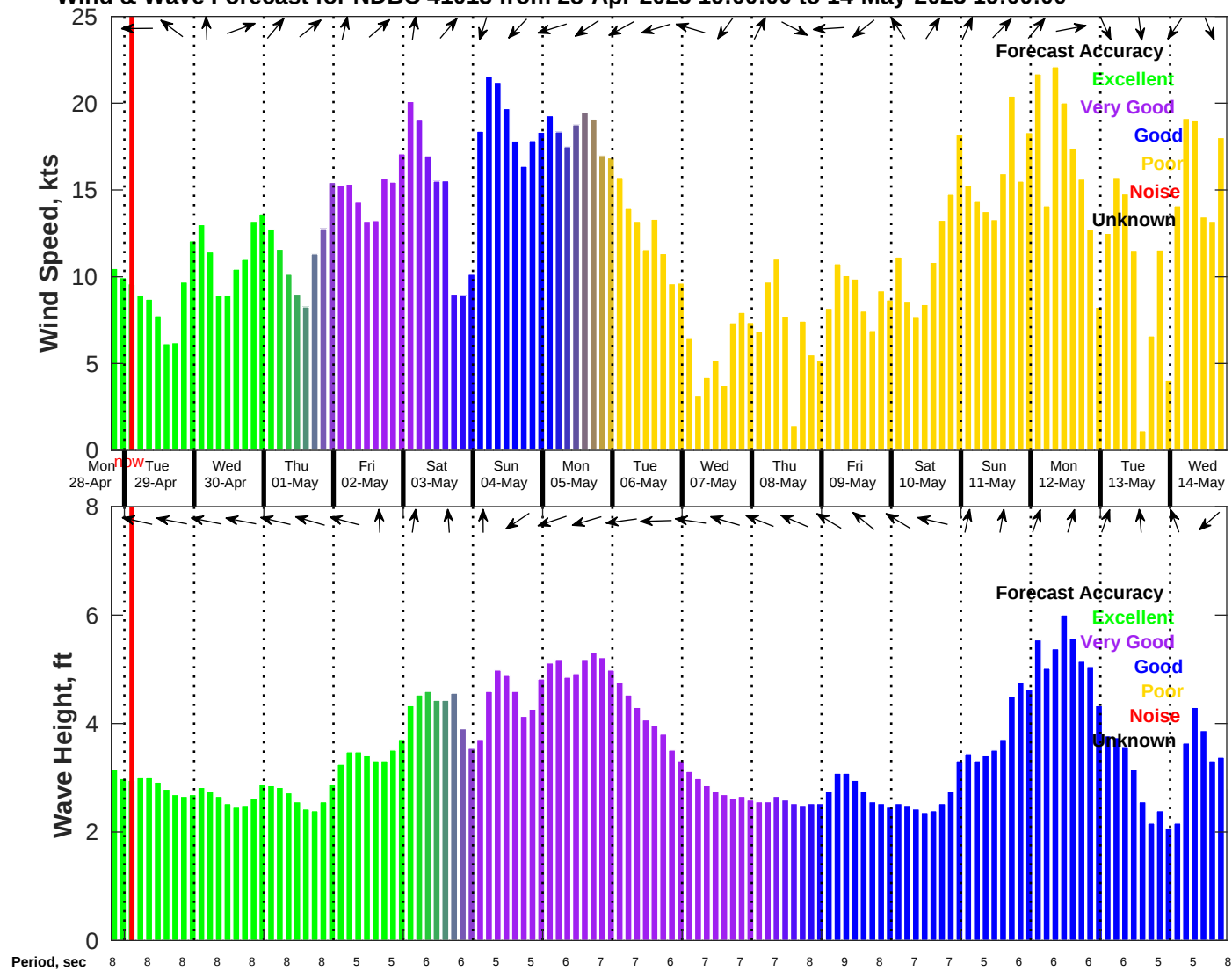
Wind & Wave Forecast for NDBC 41013 from 28-Apr-2025 19:00:00 to 14-May-2025 19:00:00
