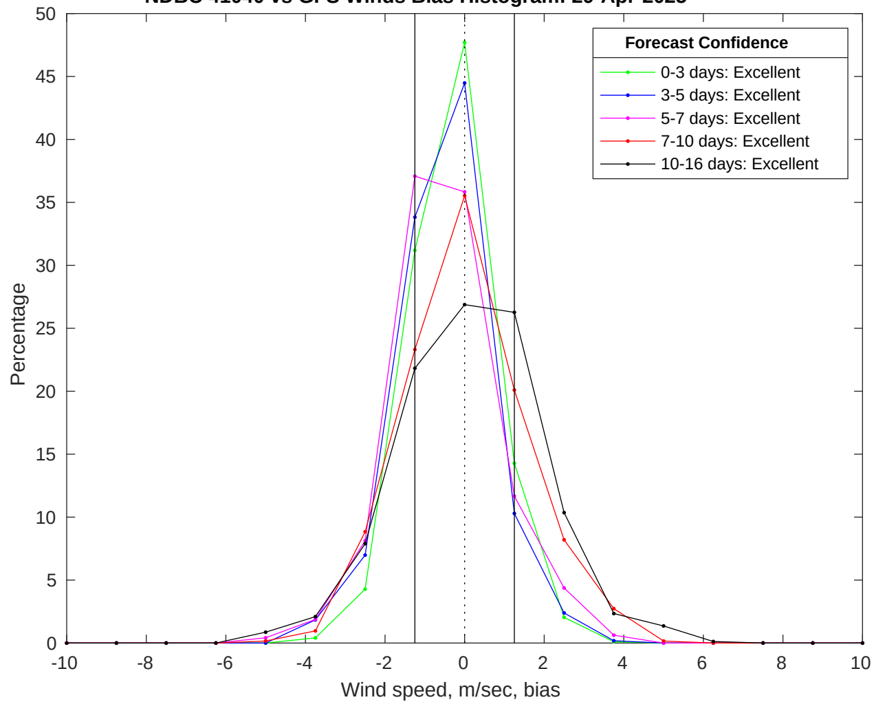
NDBC 41040 vs GFS Winds Bias Histogram: 29-Apr-2025
