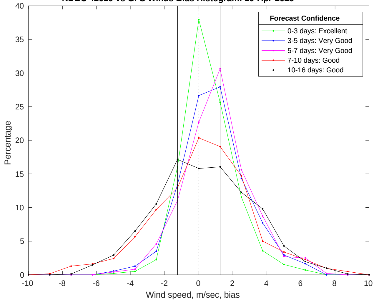
NDBC 42019 vs GFS Winds Bias Histogram: 29-Apr-2025
