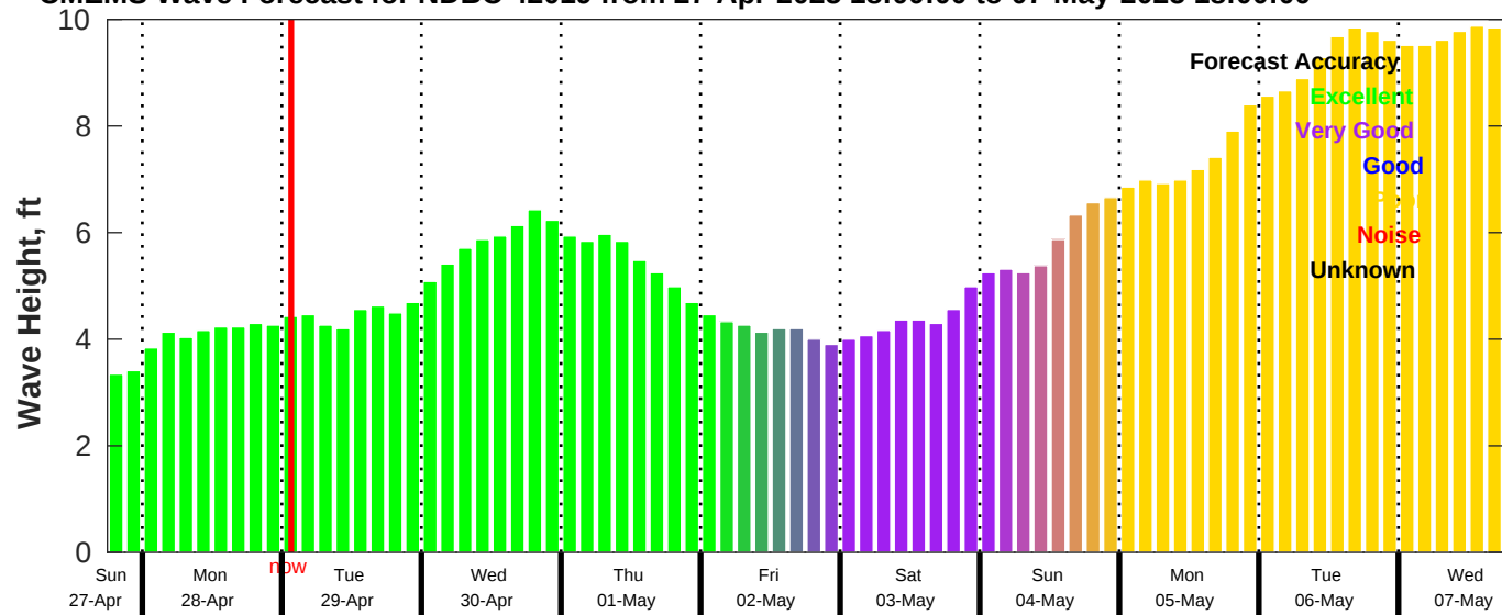
CMEMS Wave Forecast for NDBC 42019 from 27-Apr-2025 18:00:00 to 07-May-2025 18:00:00
