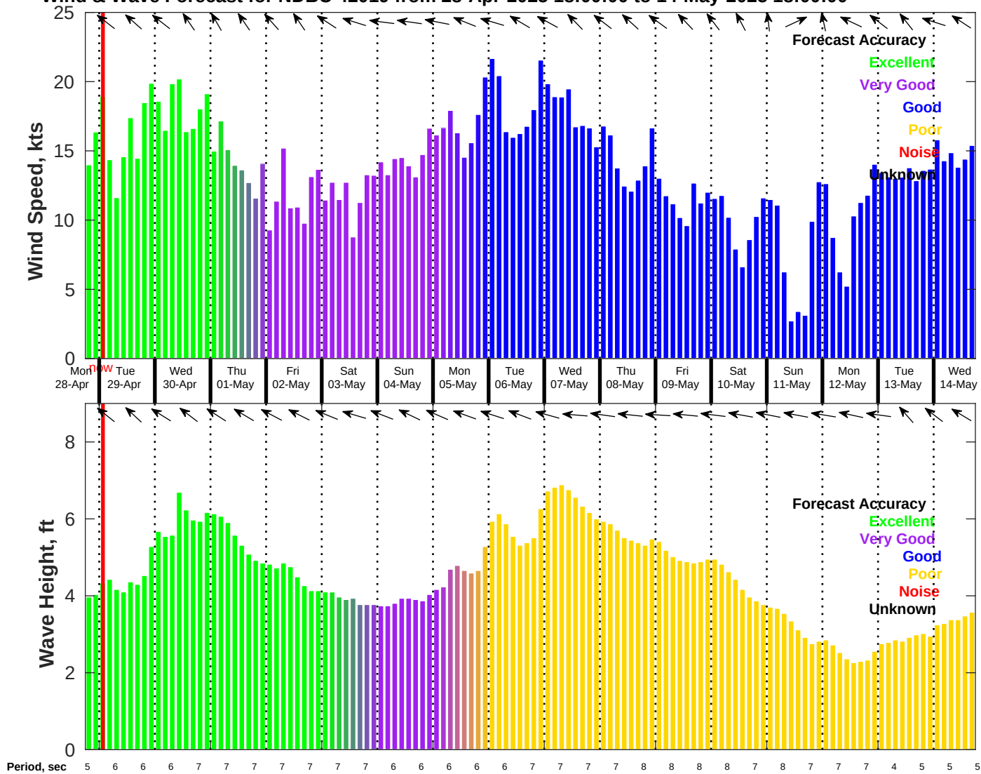
Wind & Wave Forecast for NDBC 42019 from 28-Apr-2025 18:00:00 to 14-May-2025 18:00:00
