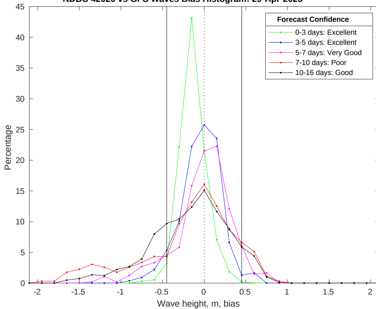
NDBC 42020 vs GFS Waves Bias Histogram: 29-Apr-2025
