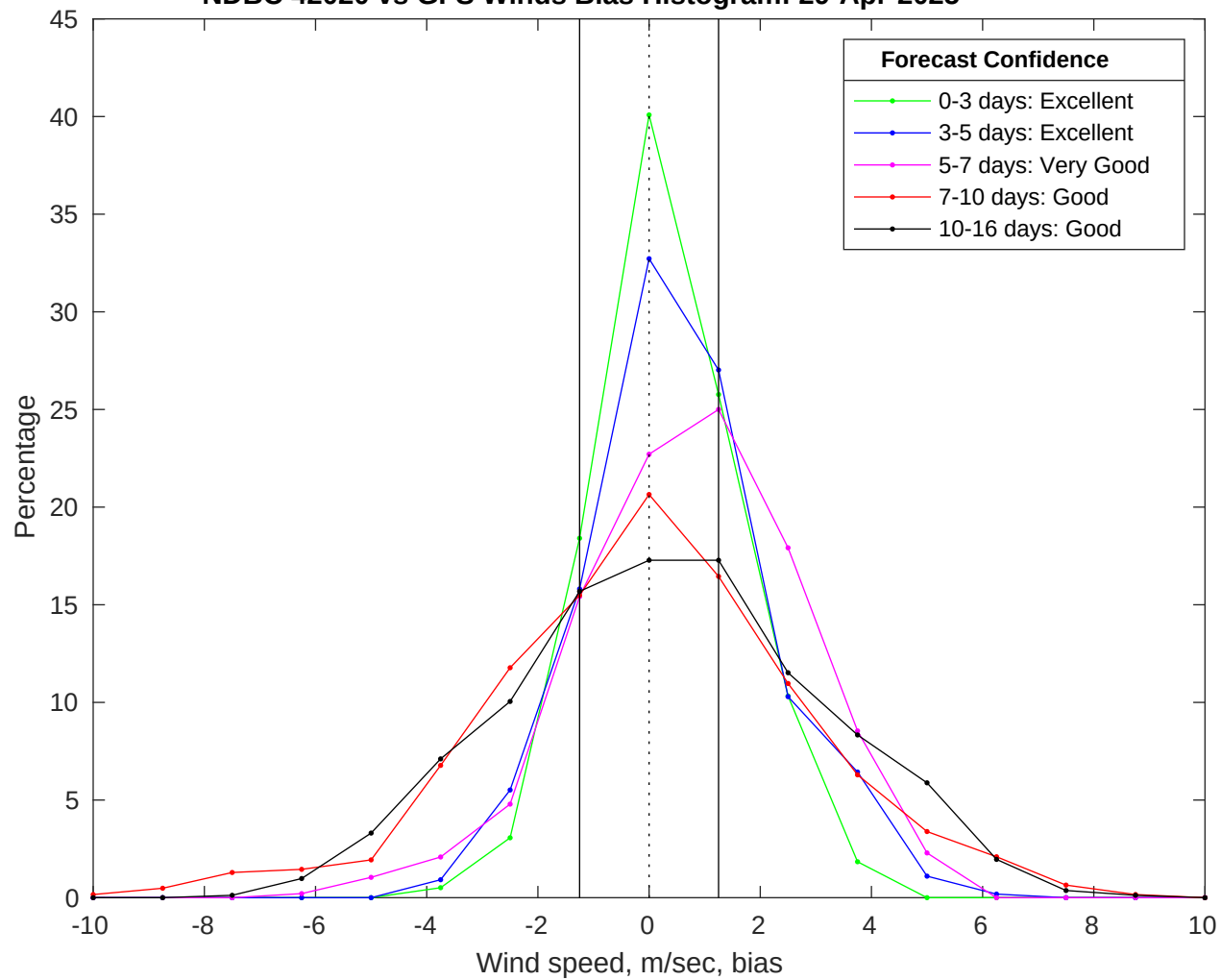
NDBC 42020 vs GFS Winds Bias Histogram: 29-Apr-2025
