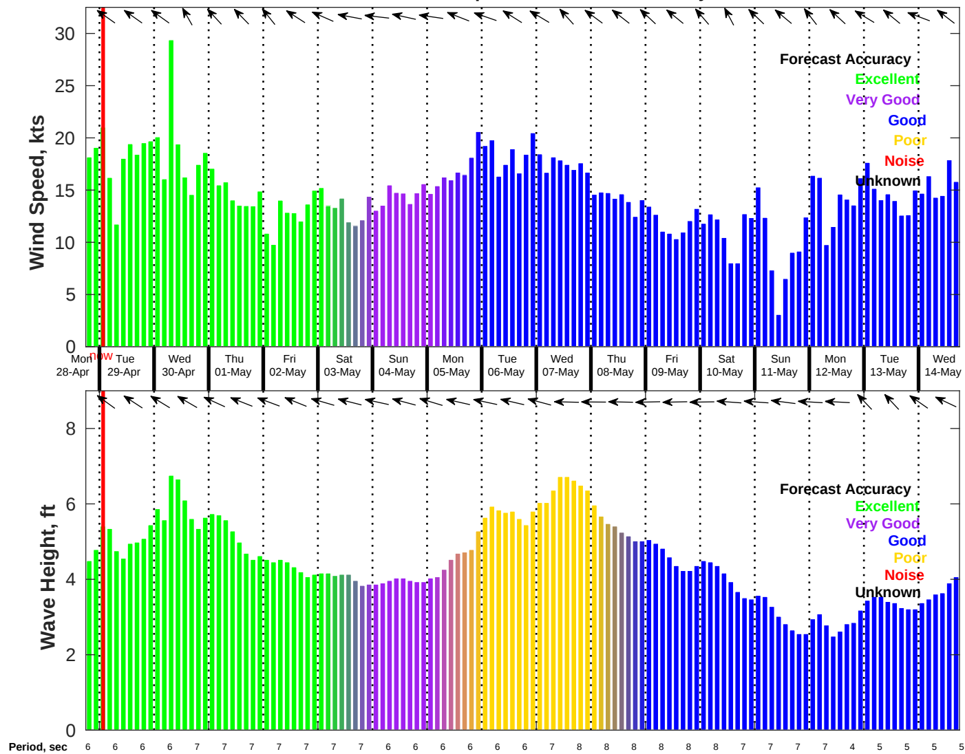
Wind & Wave Forecast for NDBC 42020 from 28-Apr-2025 18:00:00 to 14-May-2025 18:00:00
