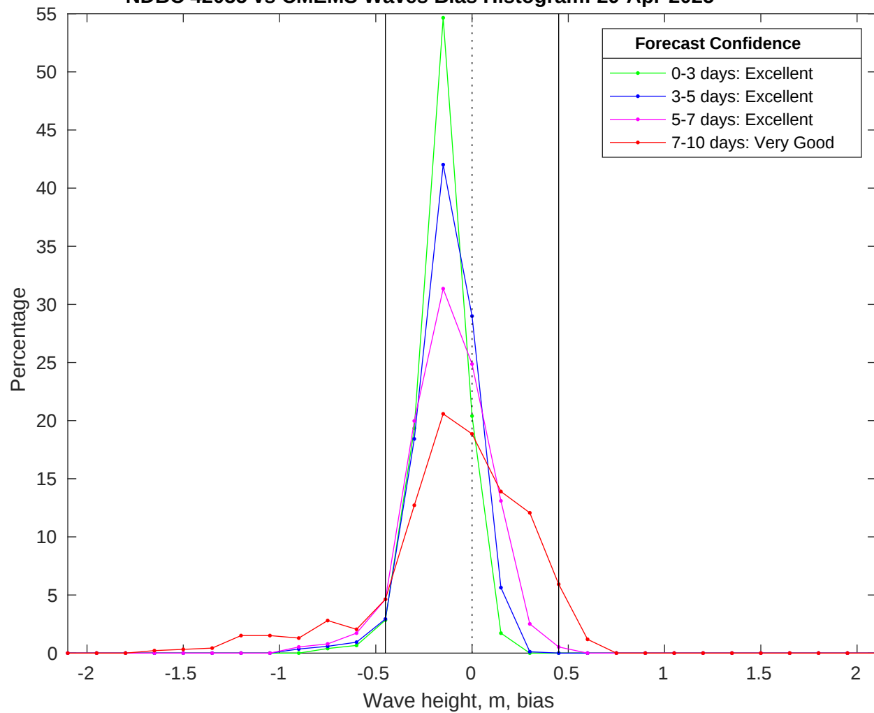
NDBC 42035 vs CMEMS Waves Bias Histogram: 29-Apr-2025
