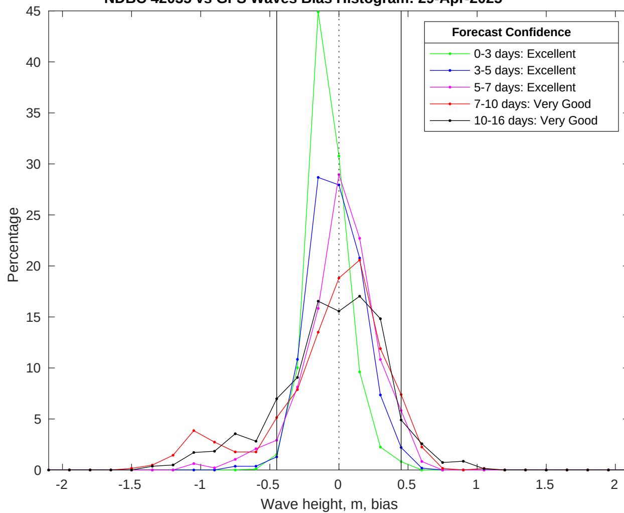
NDBC 42035 vs GFS Waves Bias Histogram: 29-Apr-2025
