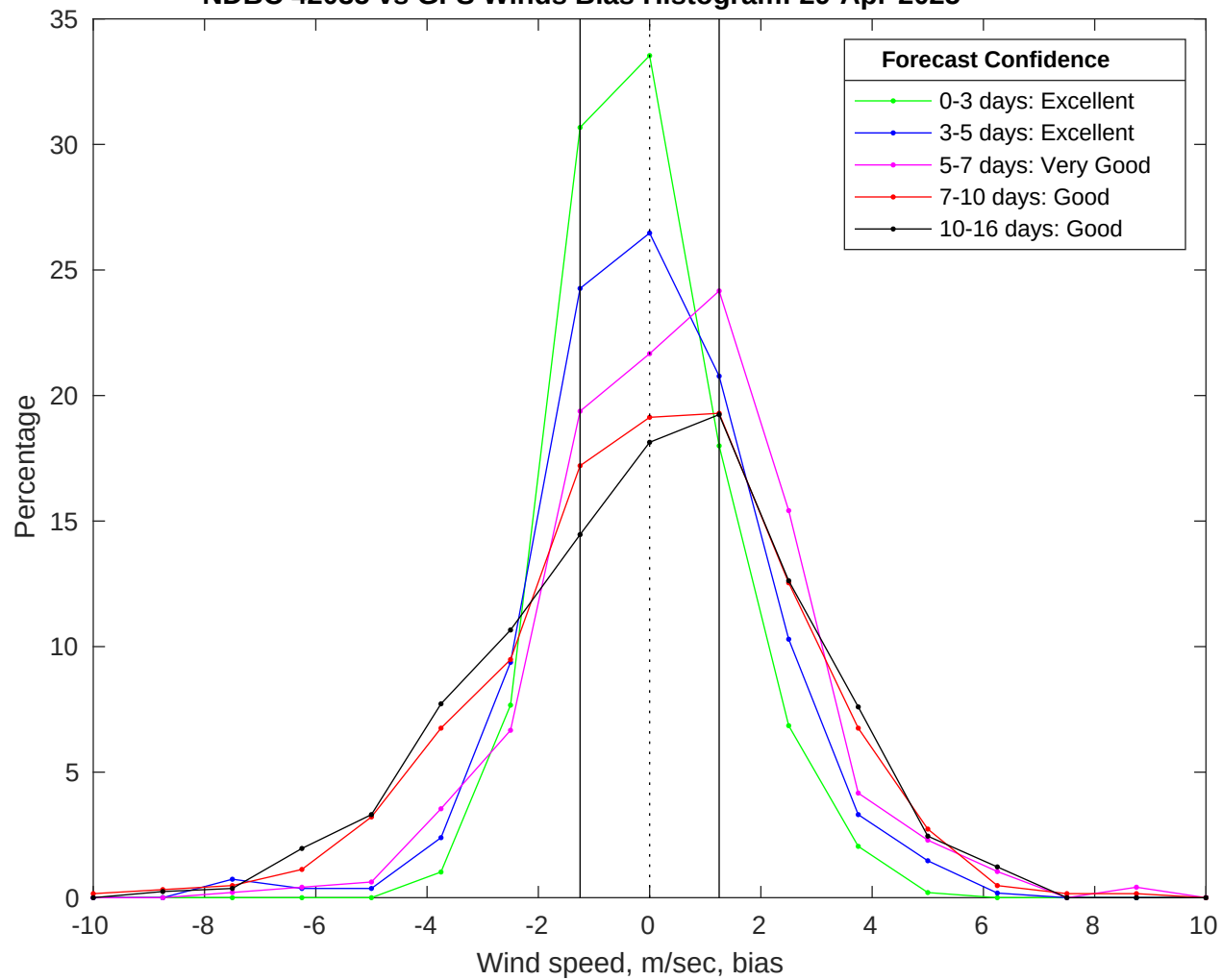
NDBC 42035 vs GFS Winds Bias Histogram: 29-Apr-2025
