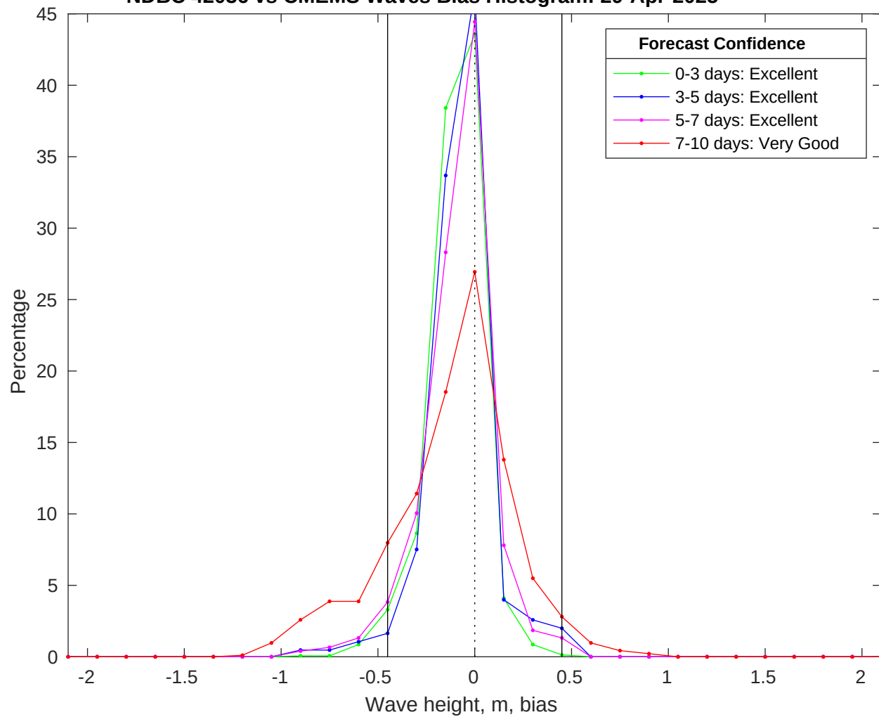
NDBC 42036 vs CMEMS Waves Bias Histogram: 29-Apr-2025
