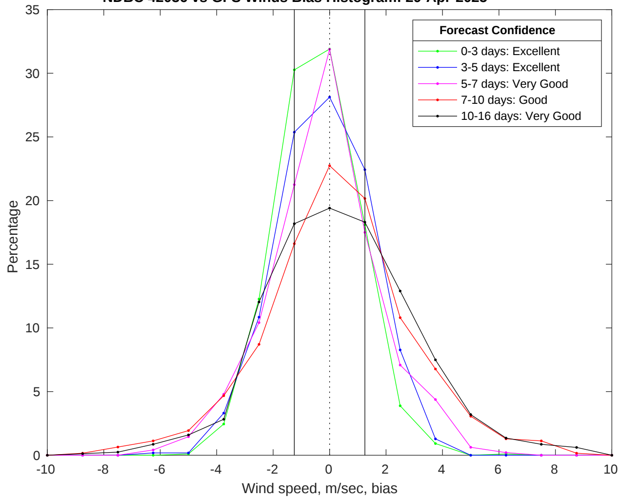
NDBC 42036 vs GFS Winds Bias Histogram: 29-Apr-2025
