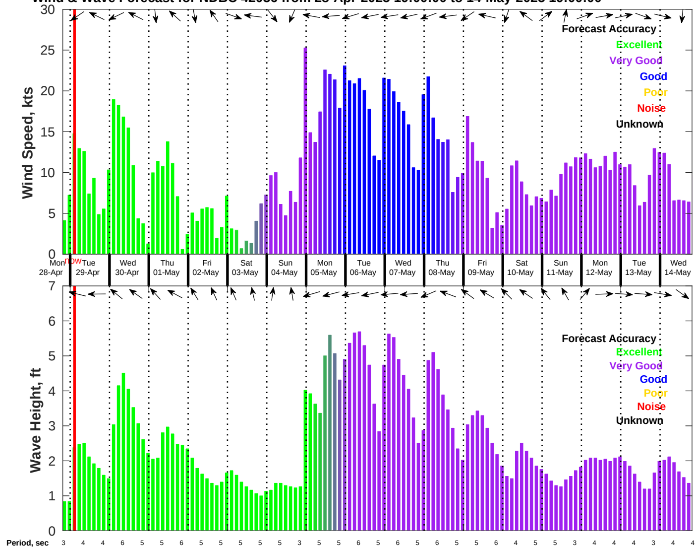
Wind & Wave Forecast for NDBC 42036 from 28-Apr-2025 19:00:00 to 14-May-2025 19:00:00
