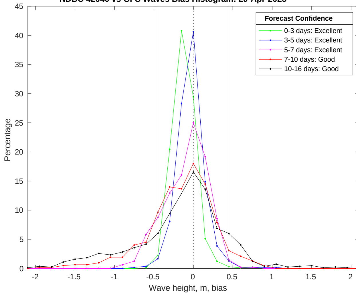
NDBC 42040 vs GFS Waves Bias Histogram: 29-Apr-2025
