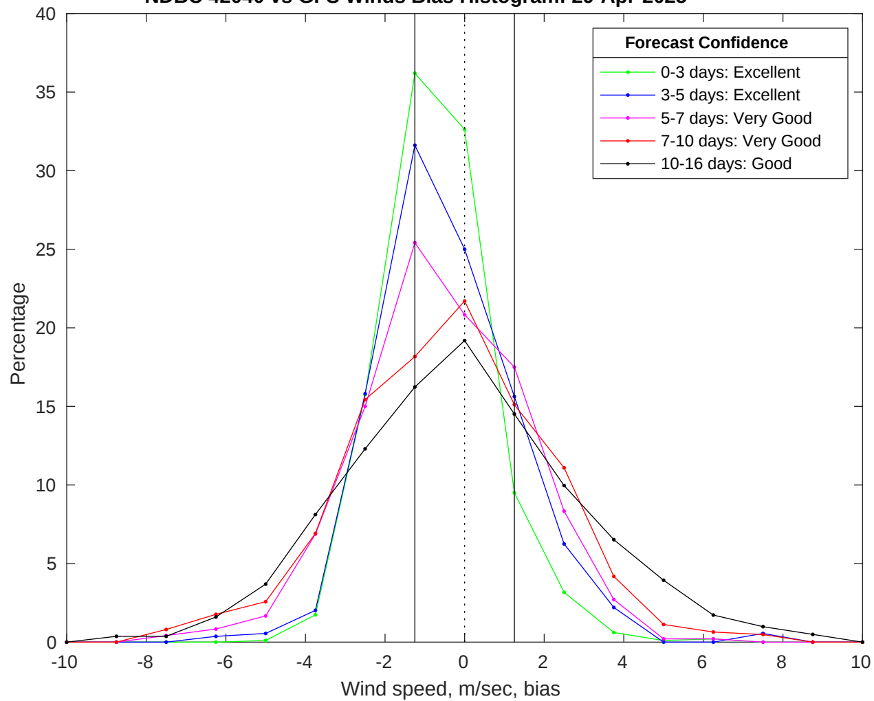
NDBC 42040 vs GFS Winds Bias Histogram: 29-Apr-2025
