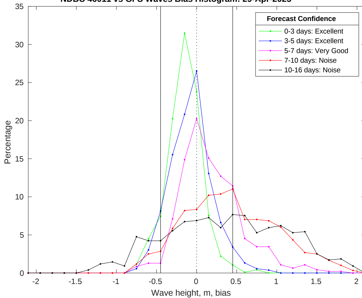
NDBC 46011 vs GFS Waves Bias Histogram: 29-Apr-2025
