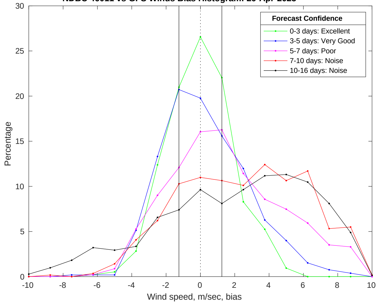
NDBC 46011 vs GFS Winds Bias Histogram: 29-Apr-2025
