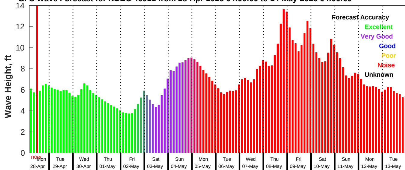
GFS Wave Forecast for NDBC 46011 from 28-Apr-2025 04:00:00 to 14-May-2025 04:00:00
