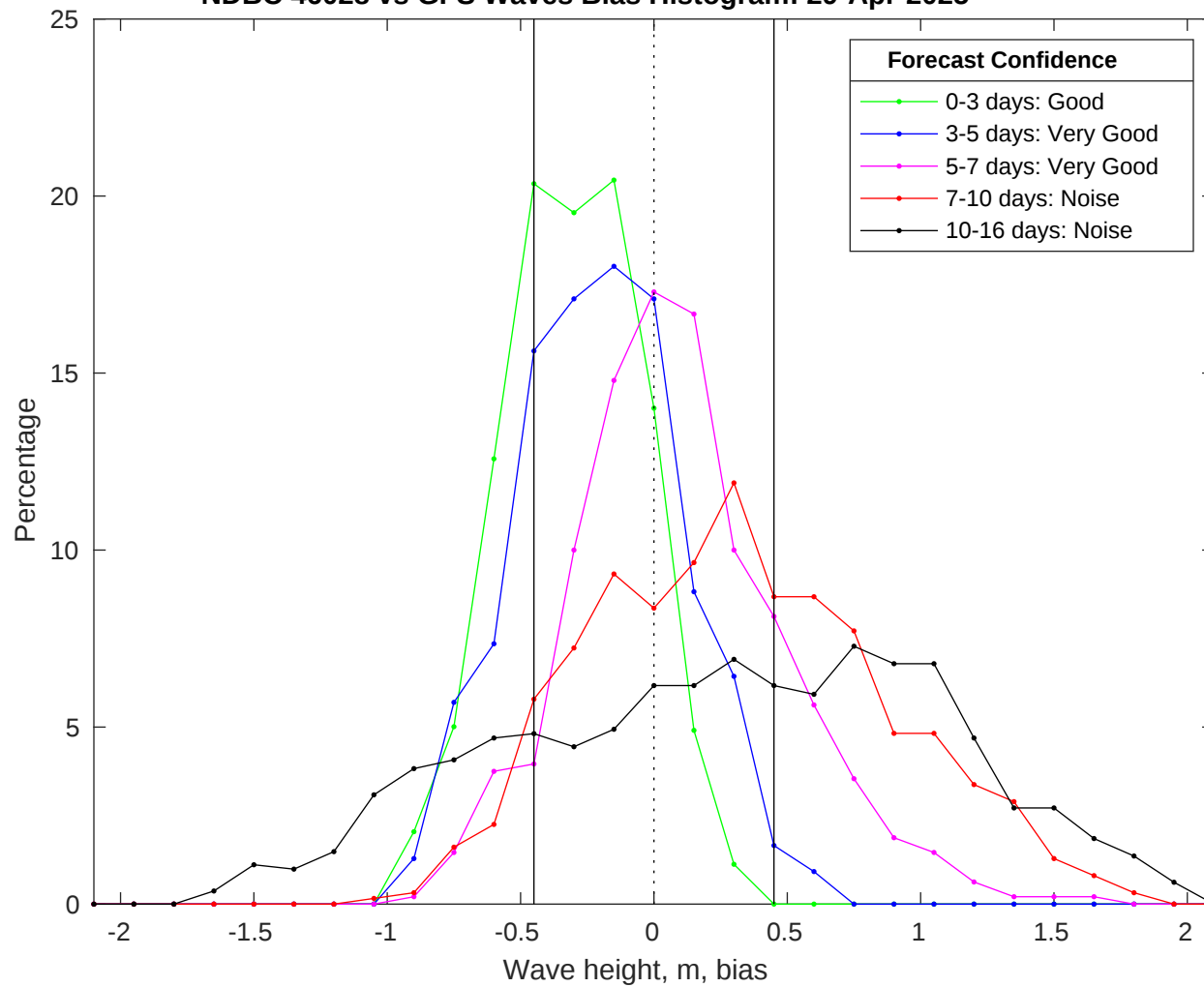
NDBC 46028 vs GFS Waves Bias Histogram: 29-Apr-2025
