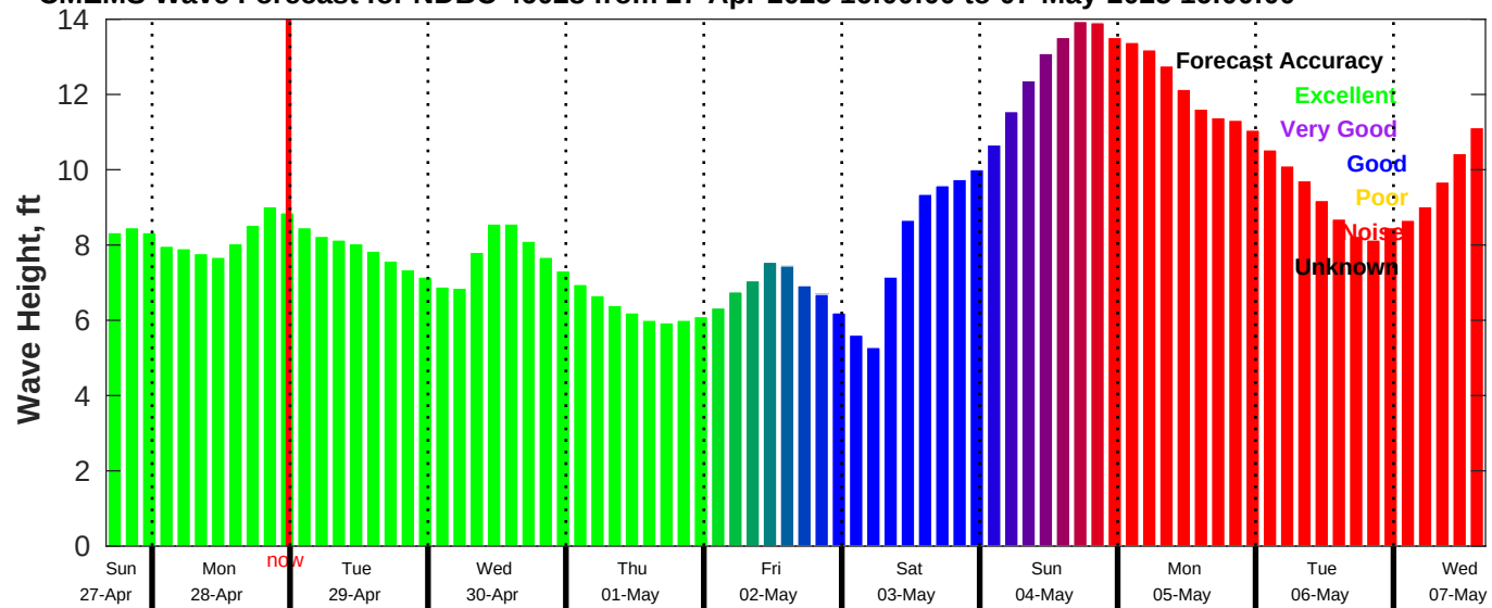
CMEMS Wave Forecast for NDBC 46028 from 27-Apr-2025 16:00:00 to 07-May-2025 16:00:00
