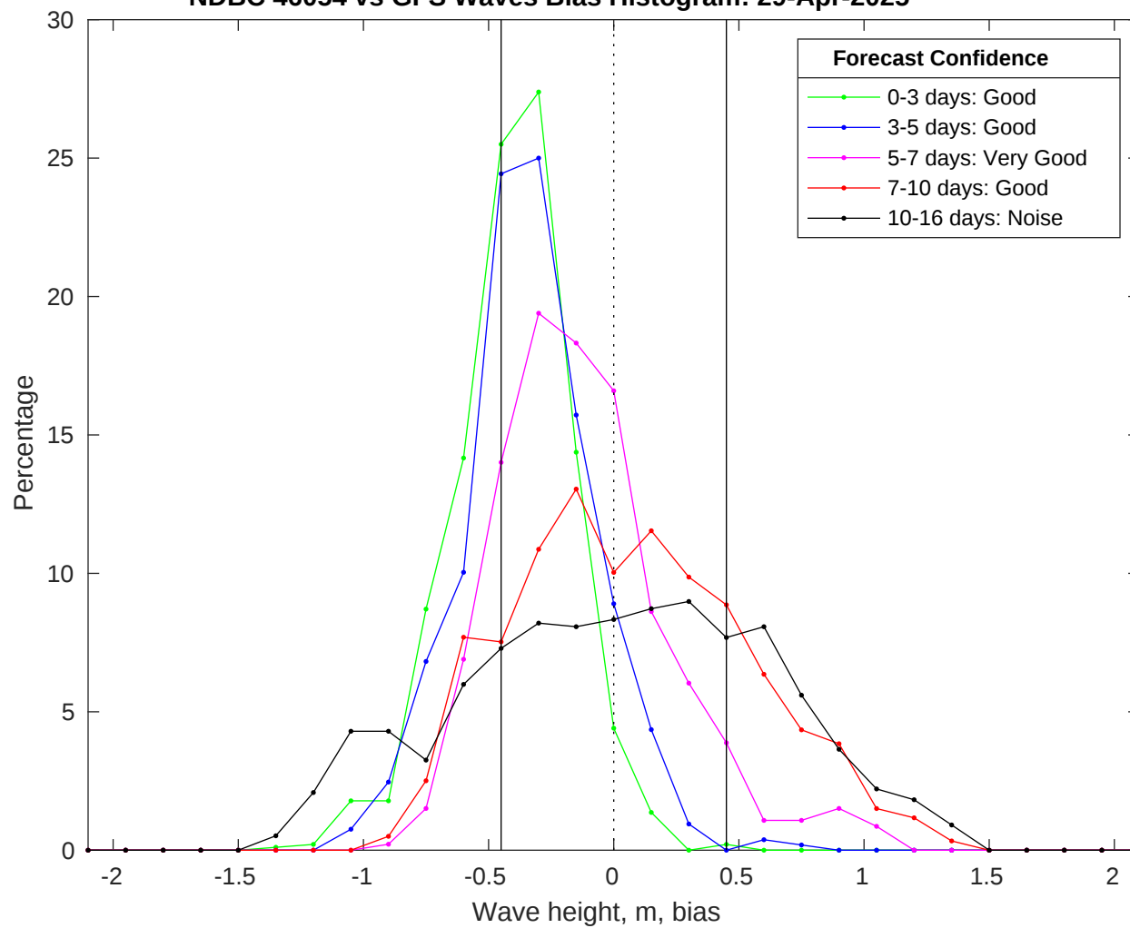
NDBC 46054 vs GFS Waves Bias Histogram: 29-Apr-2025
