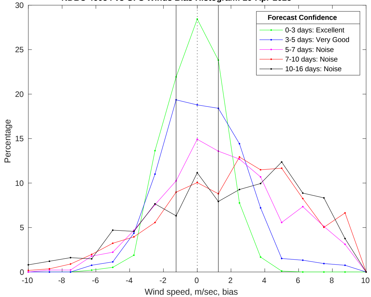
NDBC 46054 vs GFS Winds Bias Histogram: 29-Apr-2025
