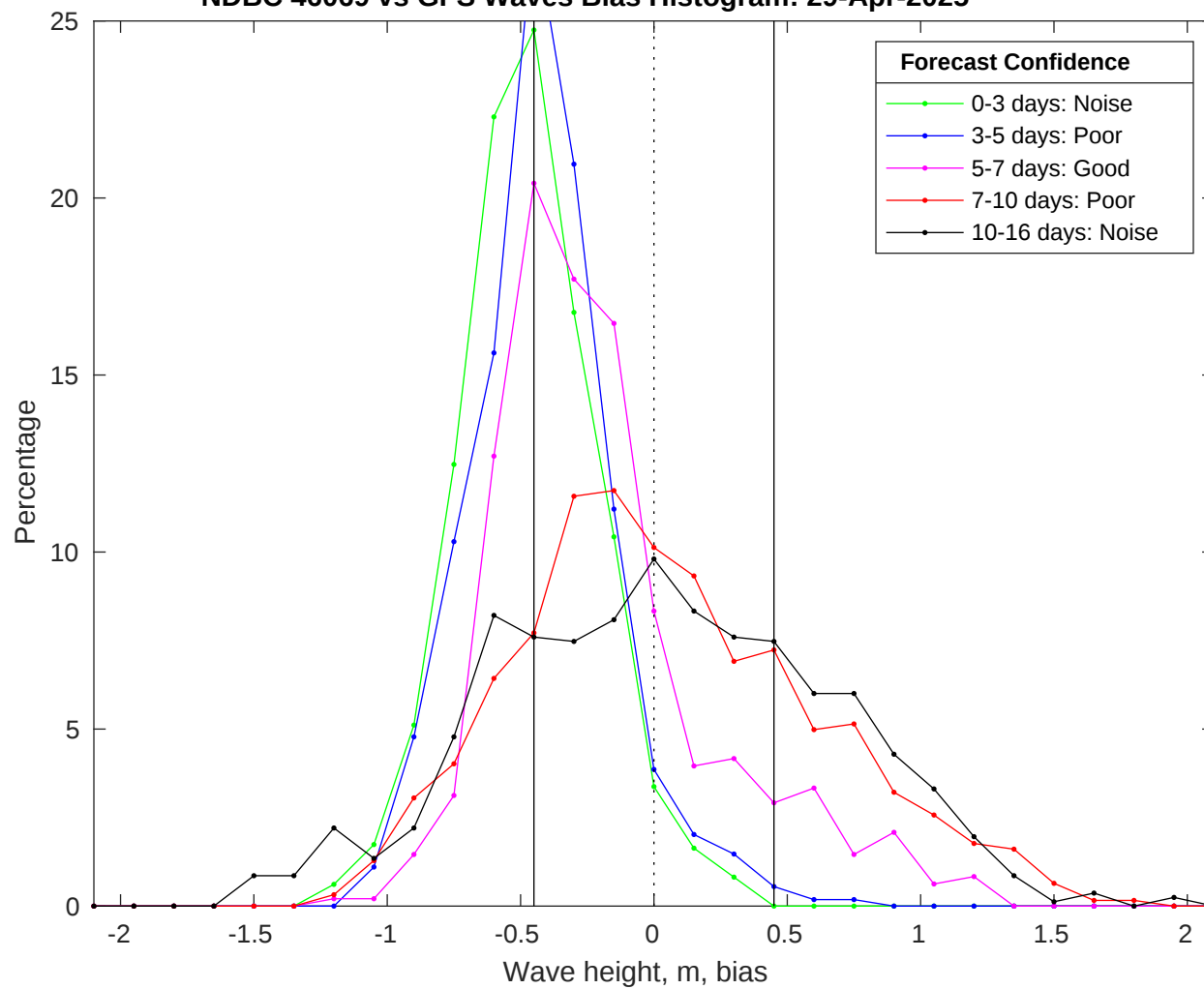
NDBC 46069 vs GFS Waves Bias Histogram: 29-Apr-2025
