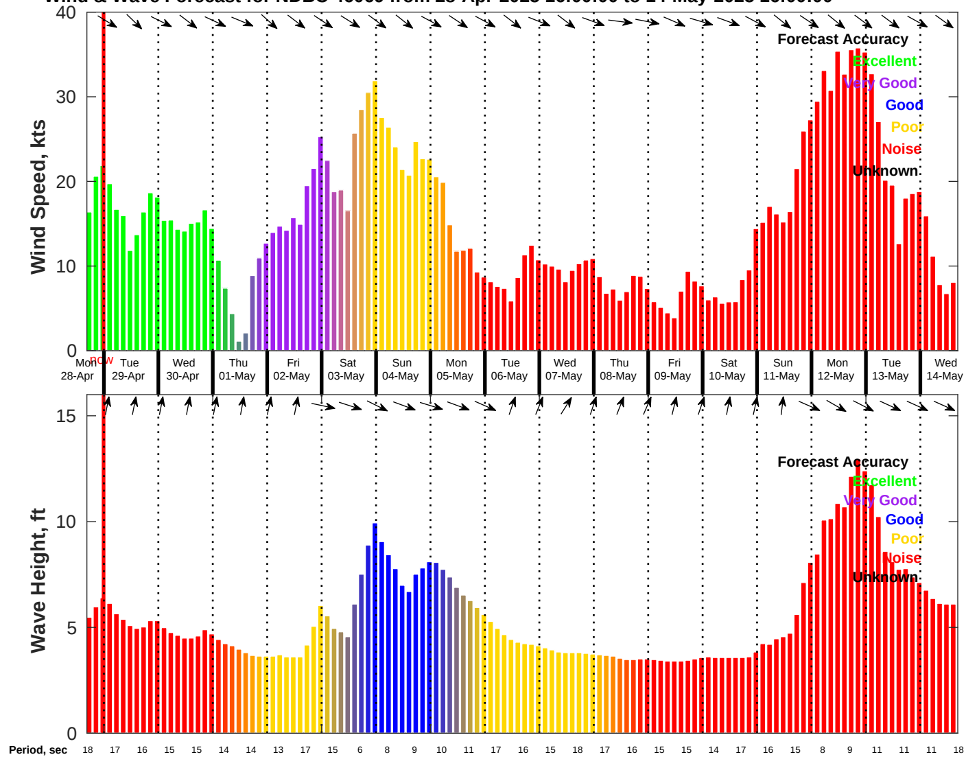
Wind & Wave Forecast for NDBC 46069 from 28-Apr-2025 16:00:00 to 14-May-2025 16:00:00
