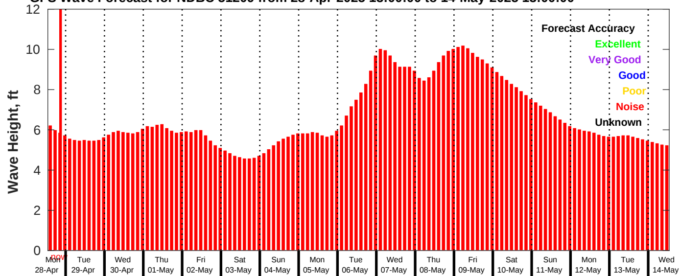
GFS Wave Forecast for NDBC 51209 from 28-Apr-2025 13:00:00 to 14-May-2025 13:00:00
