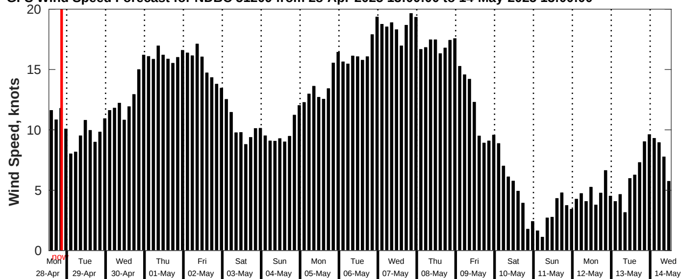
GFS Wind Speed Forecast for NDBC 51209 from 28-Apr-2025 13:00:00 to 14-May-2025 13:00:00
