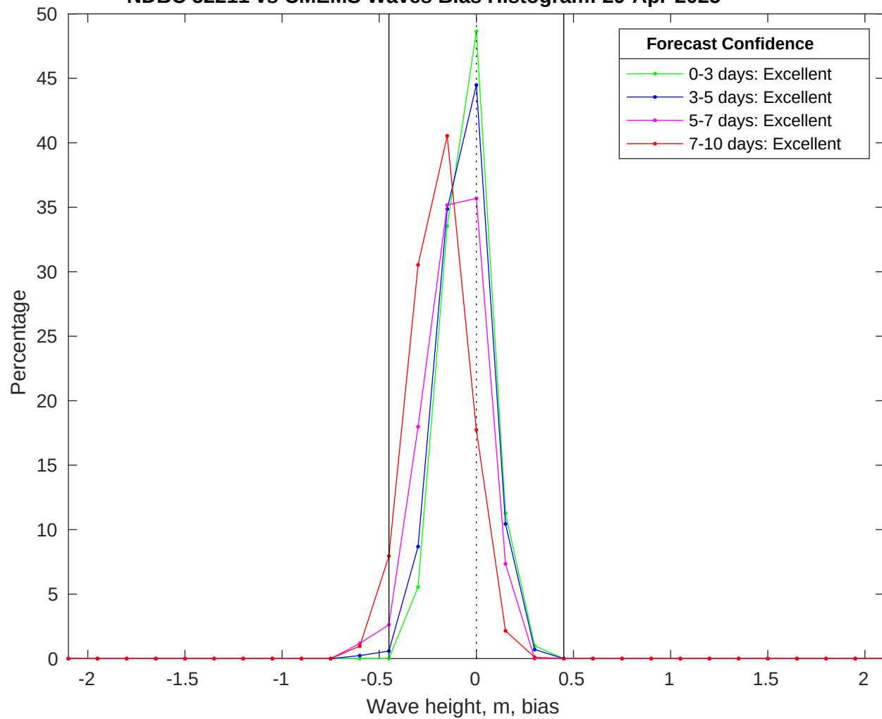
NDBC 52211 vs CMEMS Waves Bias Histogram: 29-Apr-2025
