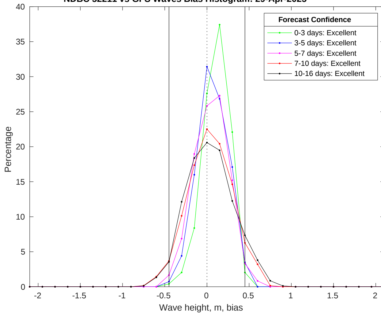
NDBC 52211 vs GFS Waves Bias Histogram: 29-Apr-2025
