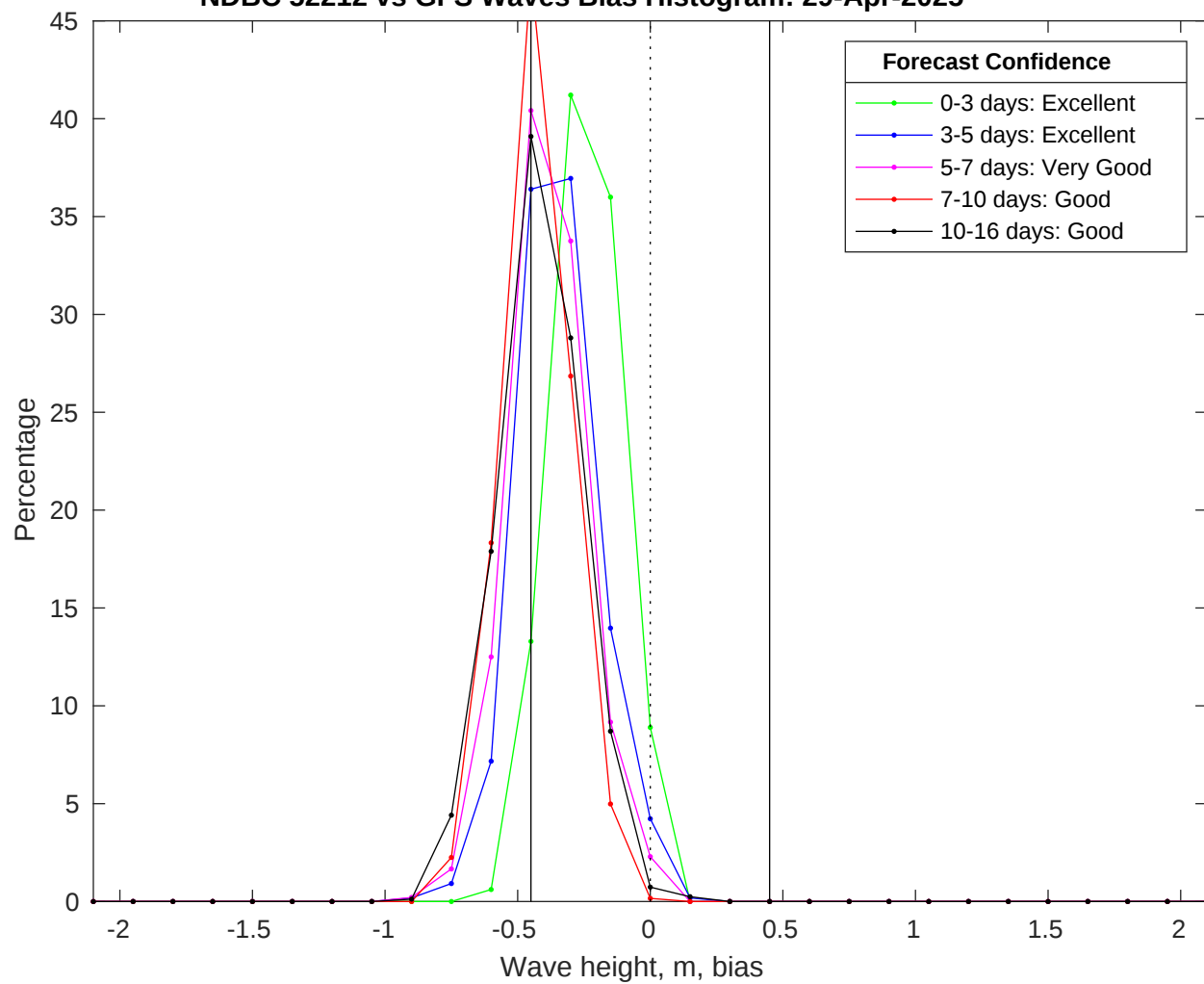
NDBC 52212 vs GFS Waves Bias Histogram: 29-Apr-2025
