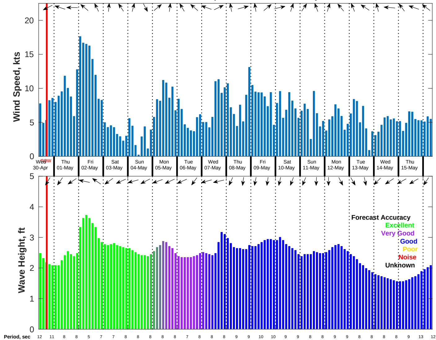
Wind & Wave Forecast for NDBC 52212 from 29-Apr-2025 09:00:00 to 15-May-2025 09:00:00
