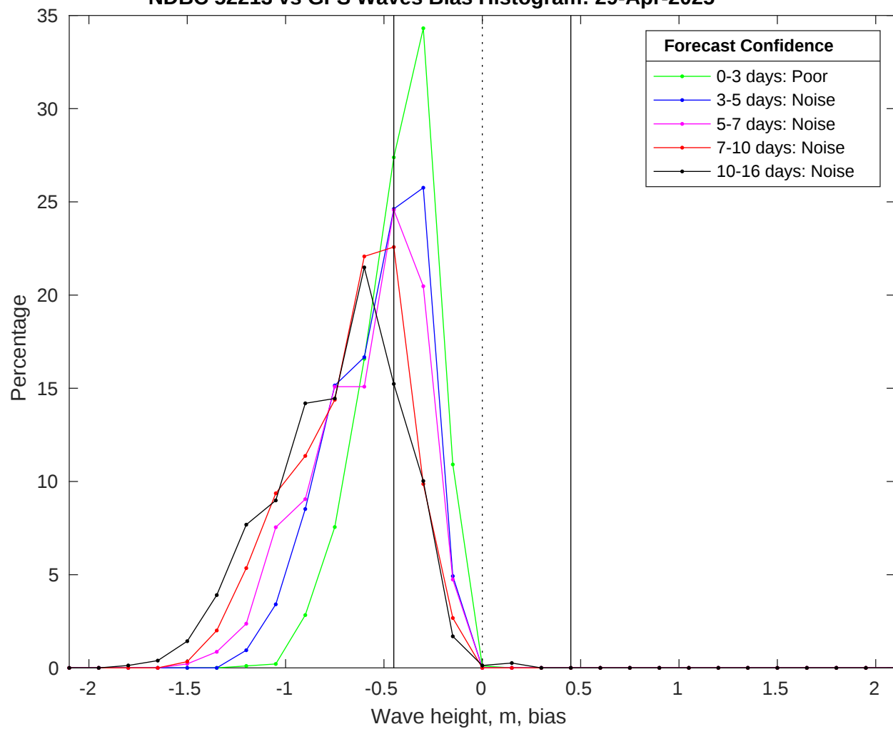
NDBC 52213 vs GFS Waves Bias Histogram: 29-Apr-2025
