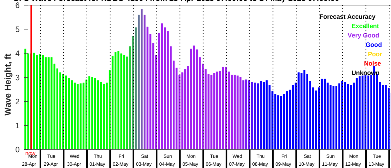
GFS Wave Forecast for NDBC 41004 from 28-Apr-2025 07:00:00 to 14-May-2025 07:00:00
