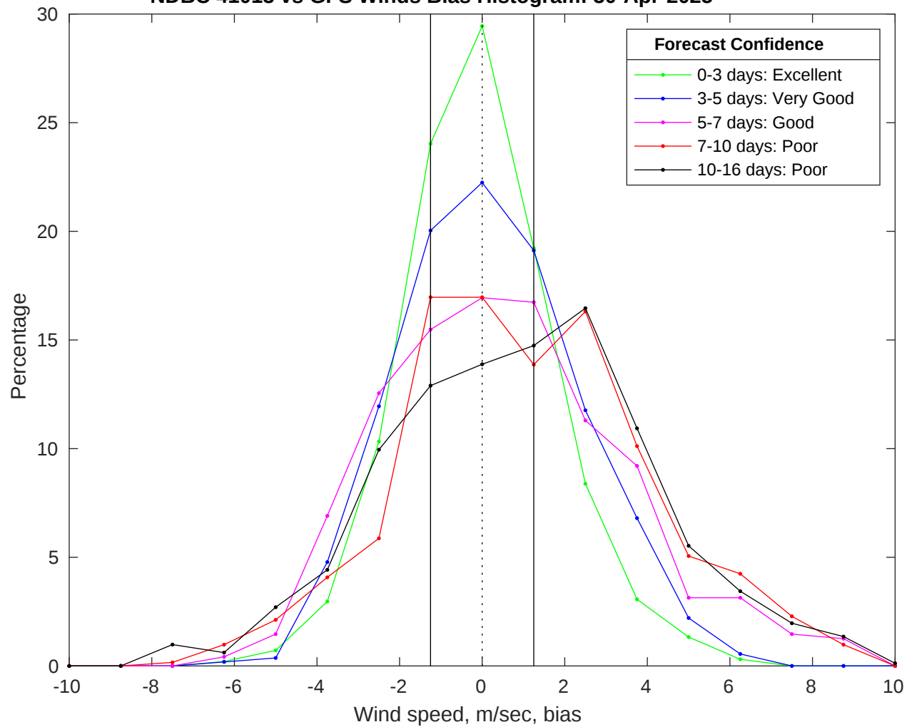
NDBC 41013 vs GFS Winds Bias Histogram: 30-Apr-2025
