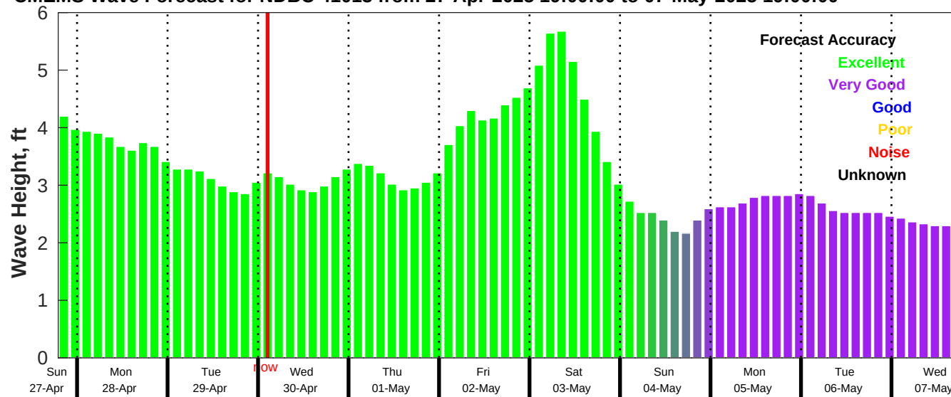
CMEMS Wave Forecast for NDBC 41013 from 27-Apr-2025 19:00:00 to 07-May-2025 19:00:00
