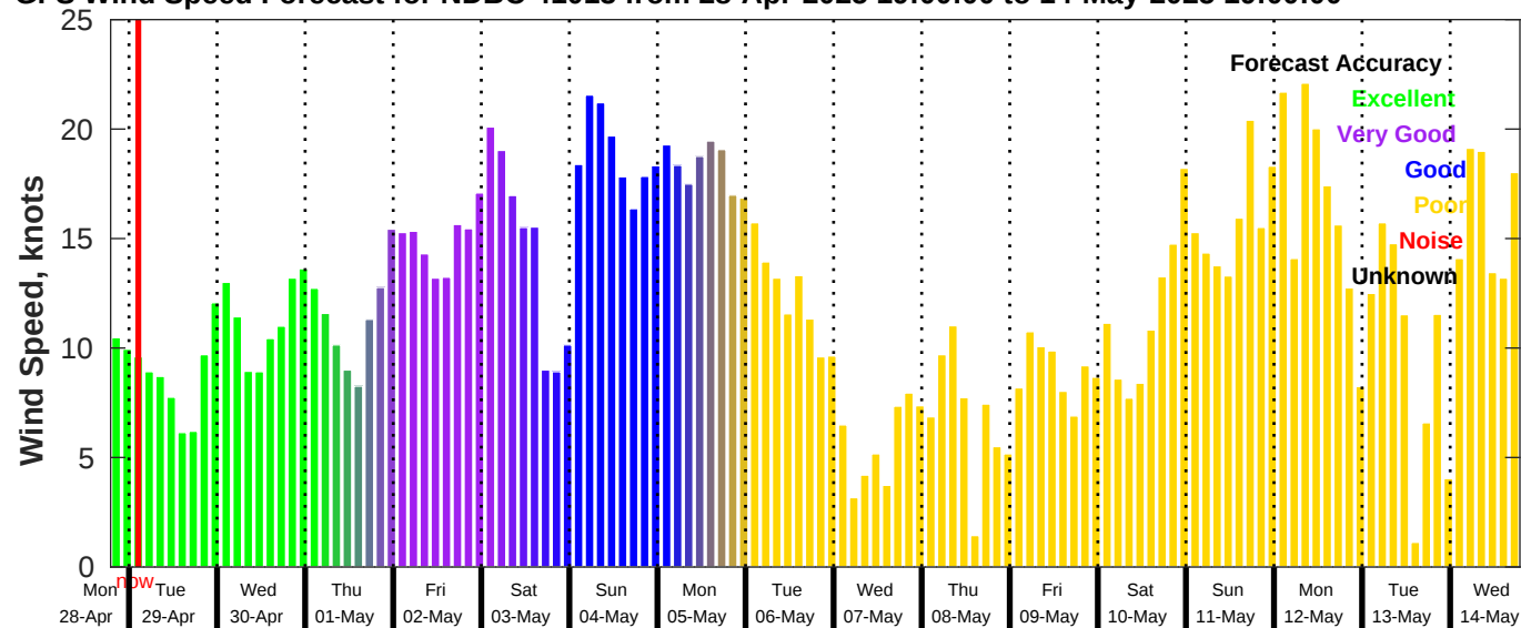
GFS Wind Speed Forecast for NDBC 41013 from 28-Apr-2025 19:00:00 to 14-May-2025 19:00:00
