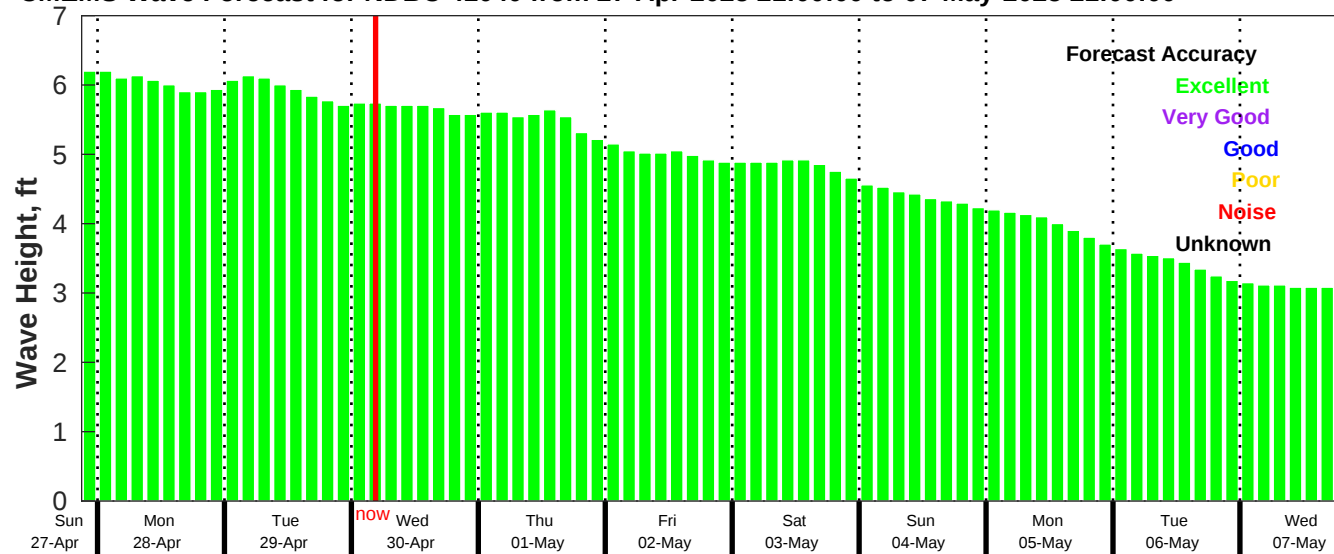
CMEMS Wave Forecast for NDBC 41040 from 27-Apr-2025 21:00:00 to 07-May-2025 21:00:00
