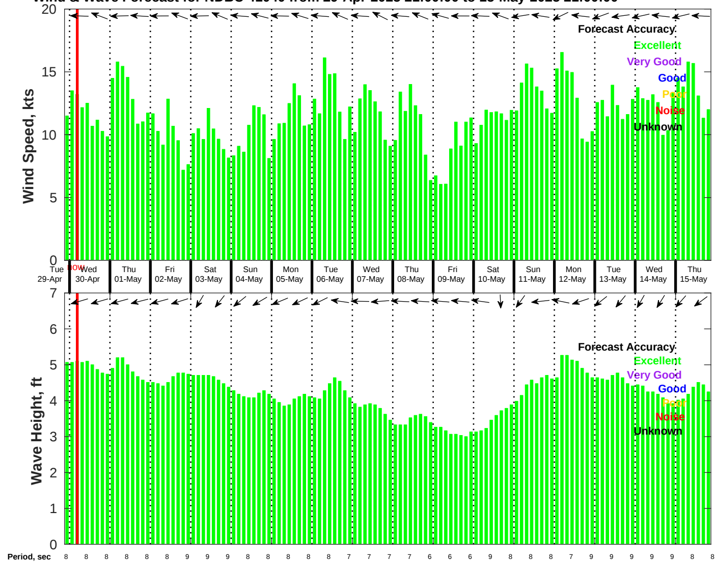
Wind & Wave Forecast for NDBC 41040 from 29-Apr-2025 21:00:00 to 15-May-2025 21:00:00
