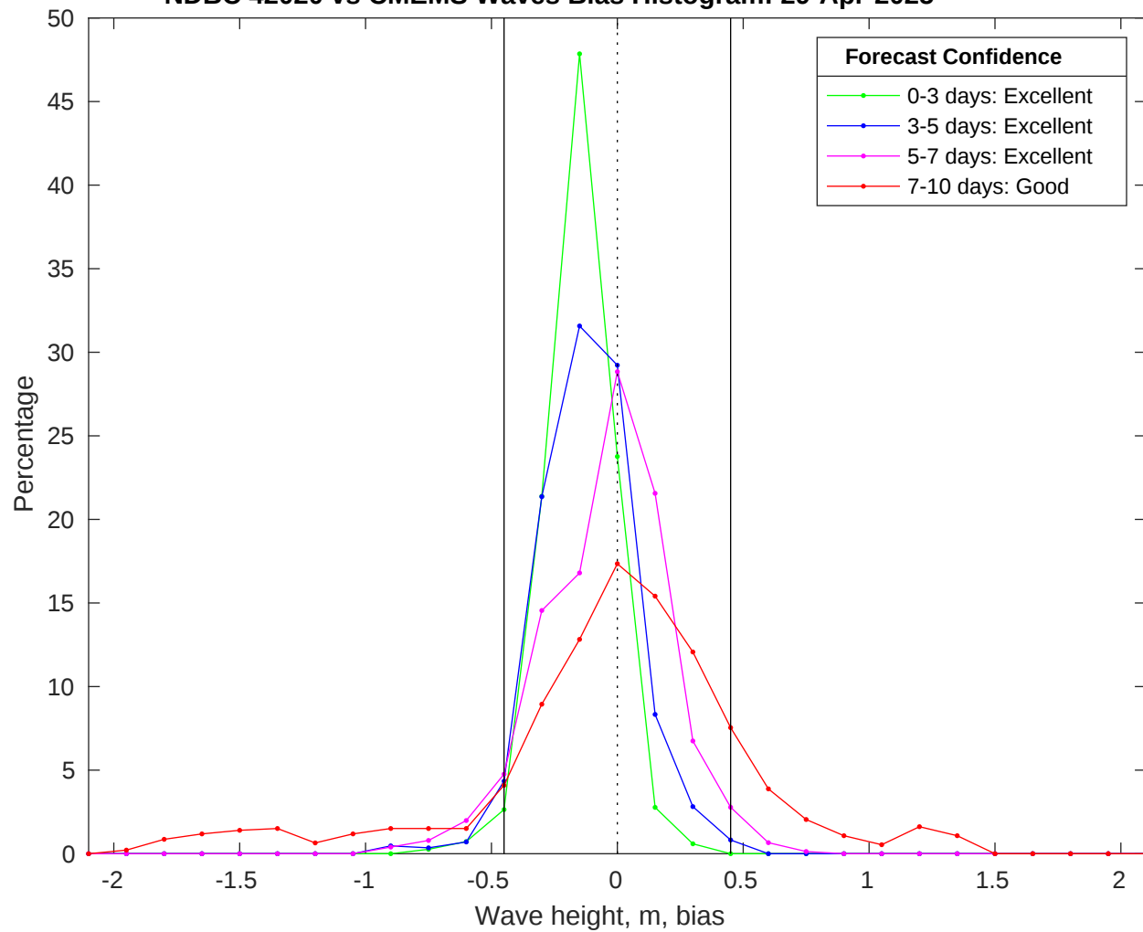
NDBC 42020 vs CMEMS Waves Bias Histogram: 29-Apr-2025
