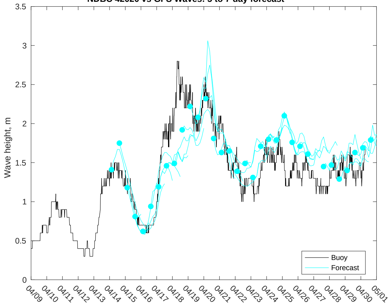
NDBC 42020 vs GFS Waves: 5 to 7 day forecast
