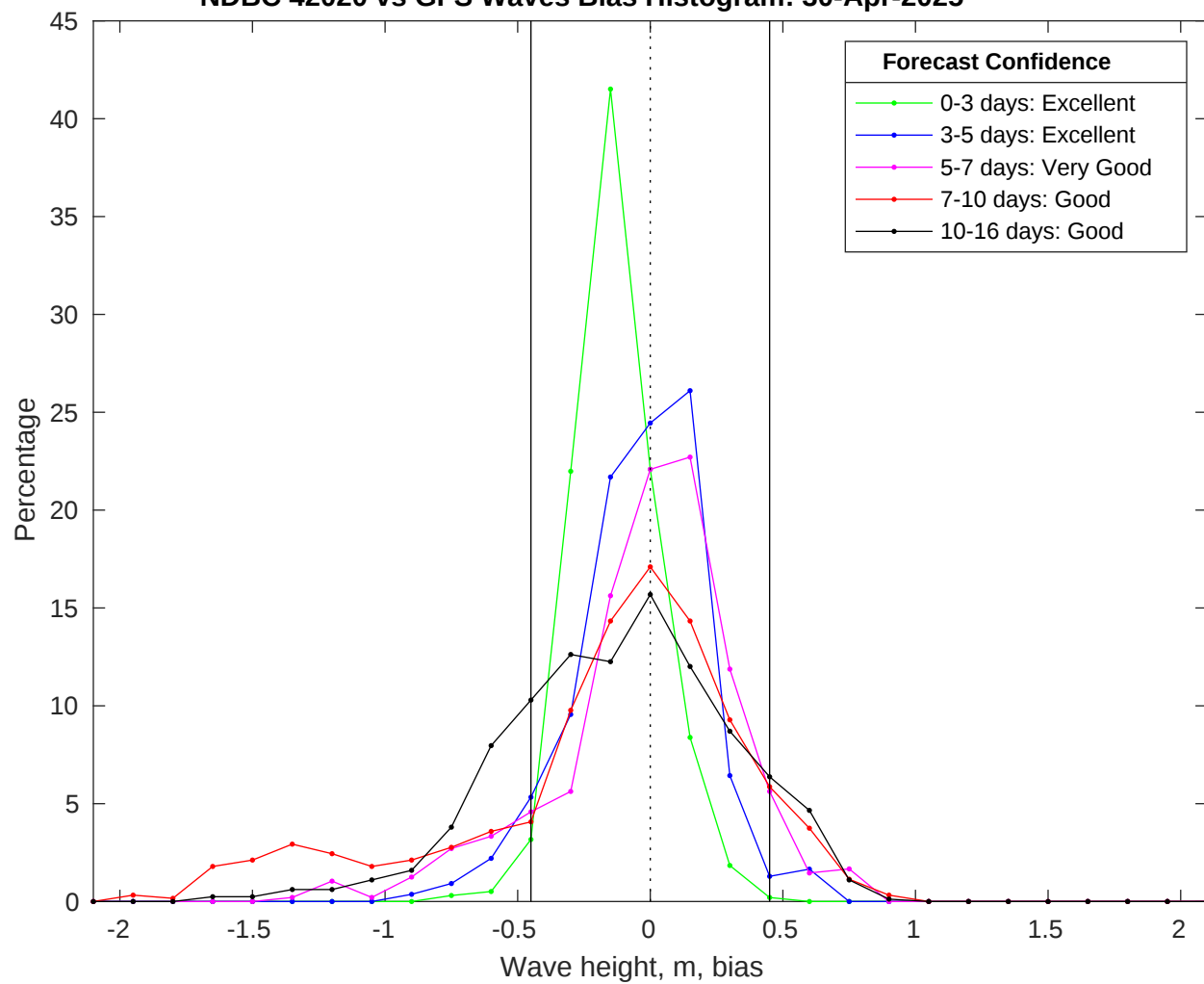
NDBC 42020 vs GFS Waves Bias Histogram: 30-Apr-2025
