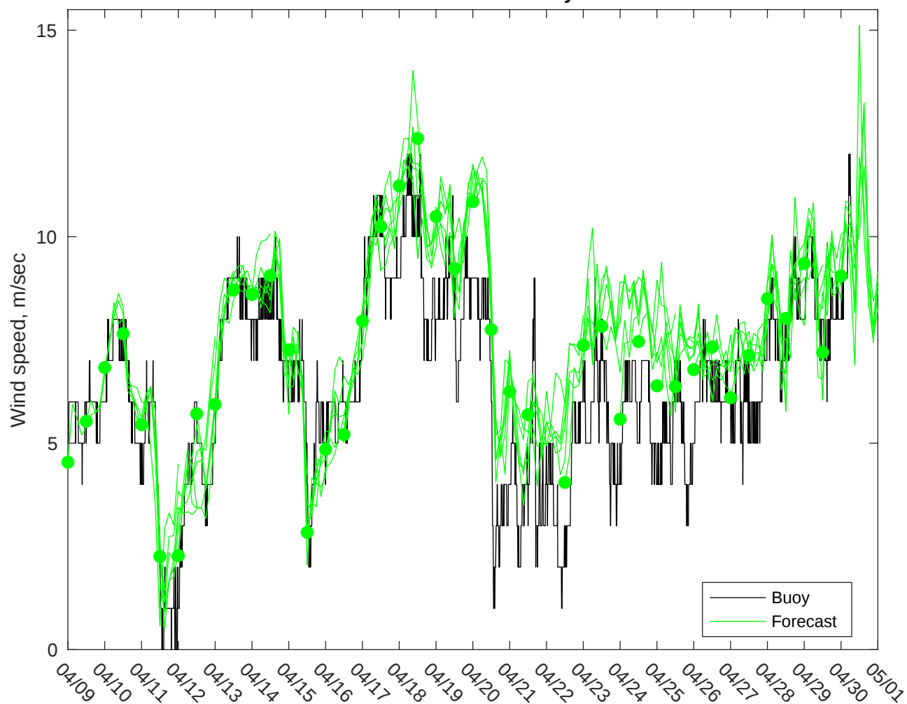
NDBC 42020 vs GFS Winds: 0 to 3 day forecast
