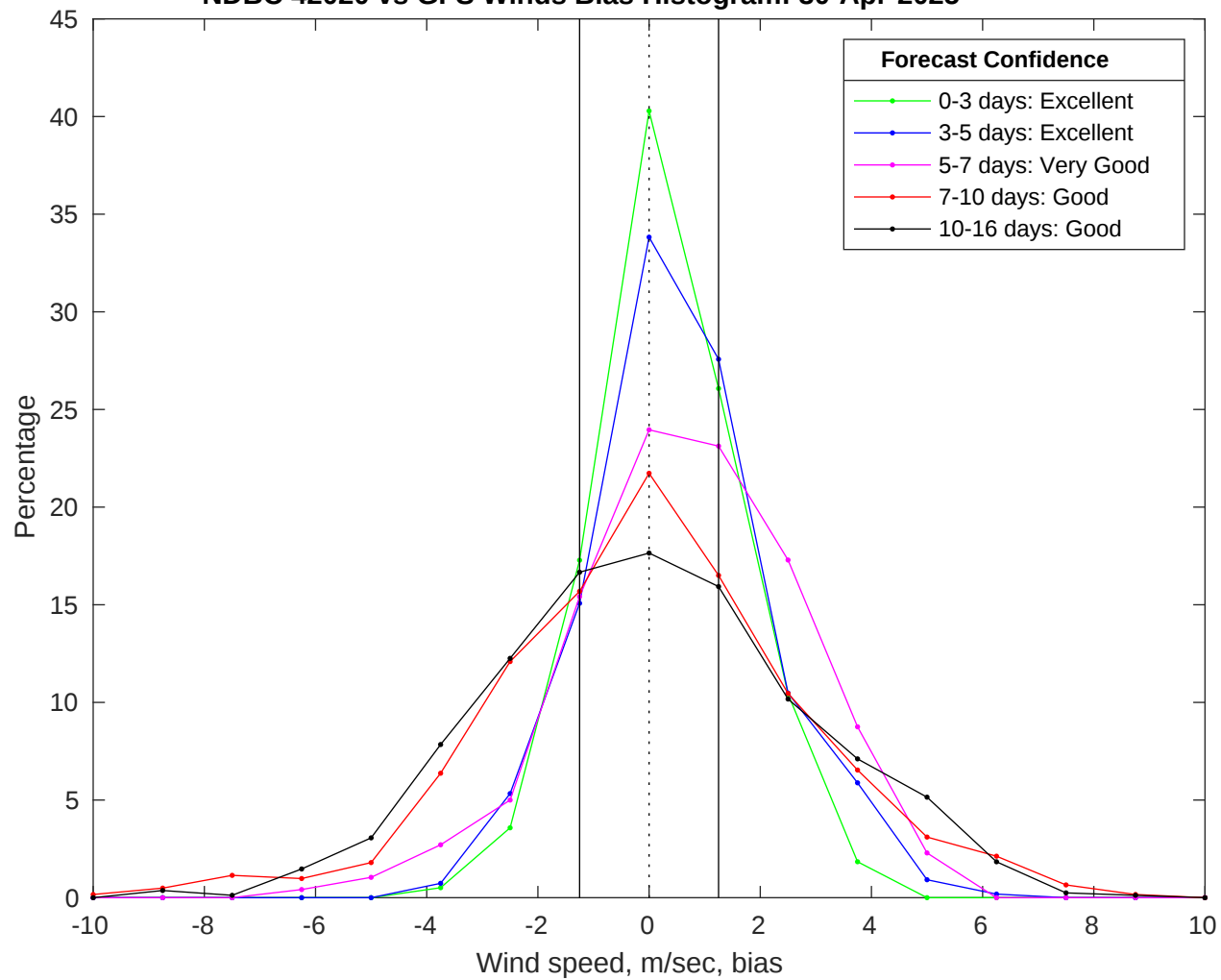
NDBC 42020 vs GFS Winds Bias Histogram: 30-Apr-2025
