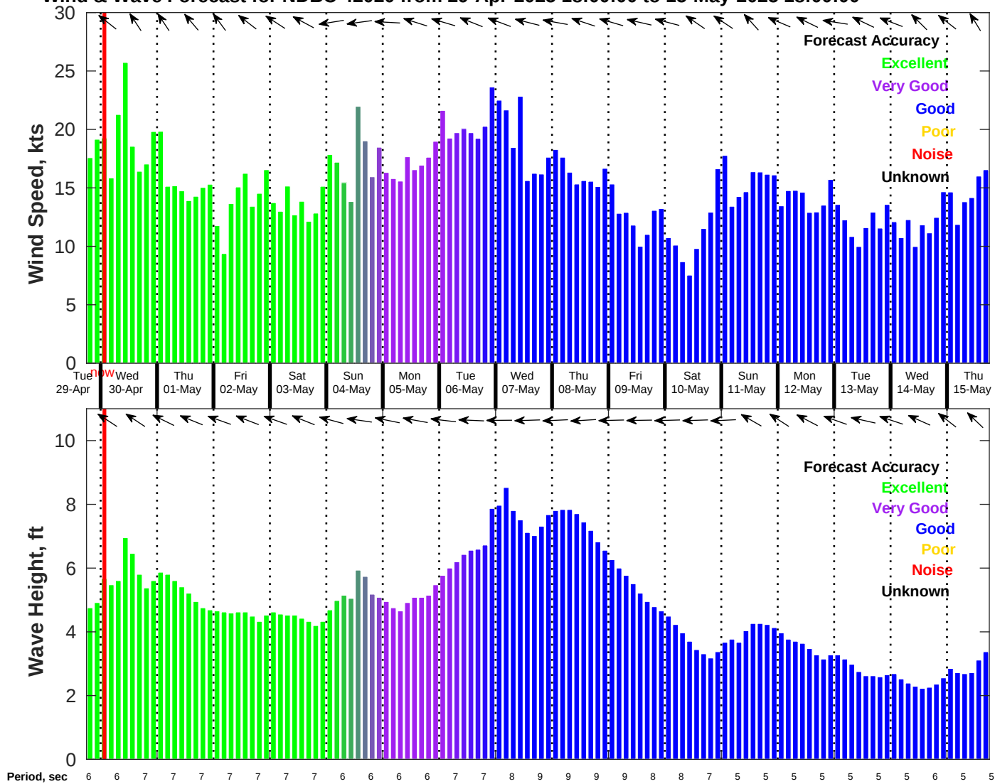
Wind & Wave Forecast for NDBC 42020 from 29-Apr-2025 18:00:00 to 15-May-2025 18:00:00
