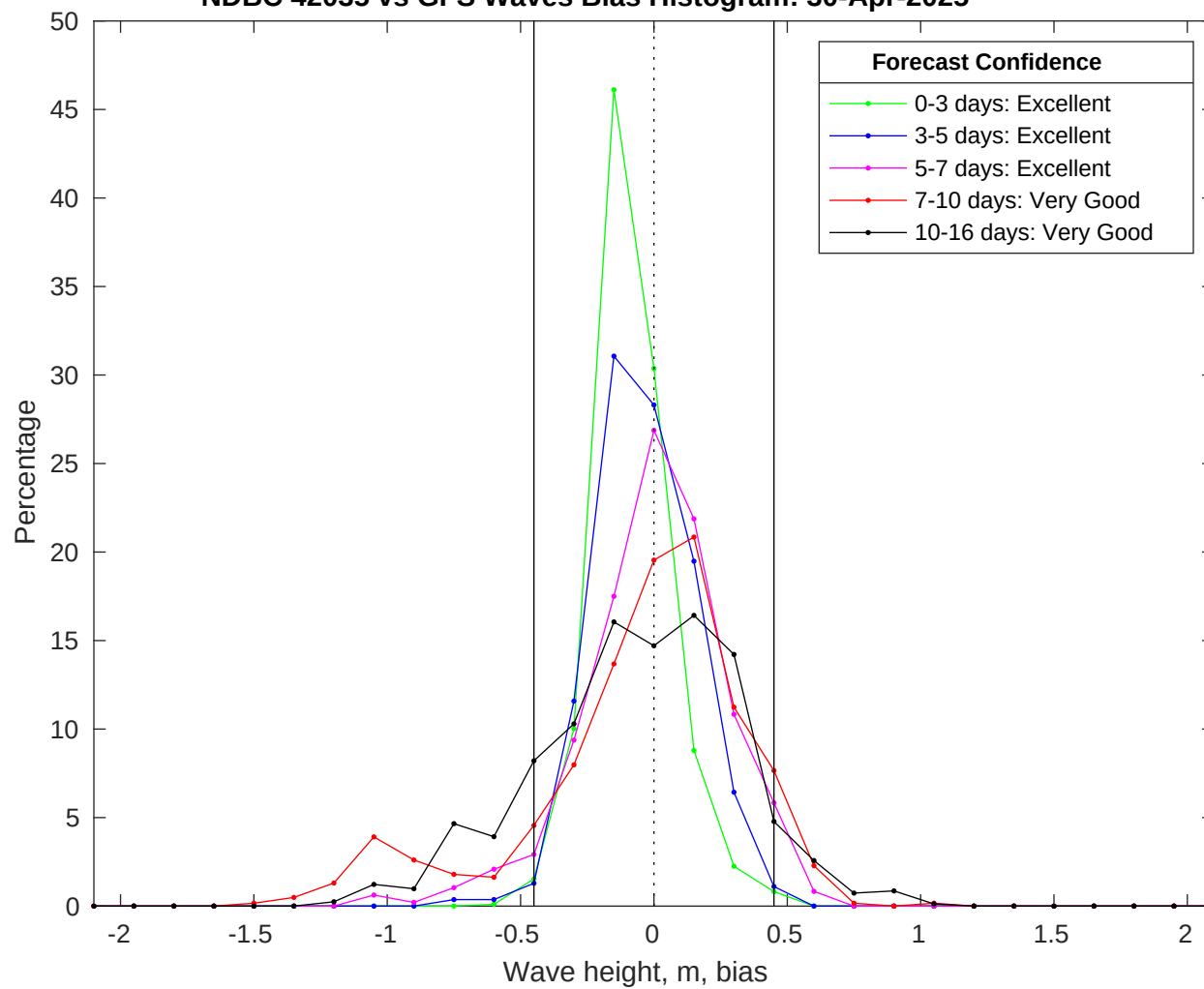
NDBC 42035 vs GFS Waves Bias Histogram: 30-Apr-2025
