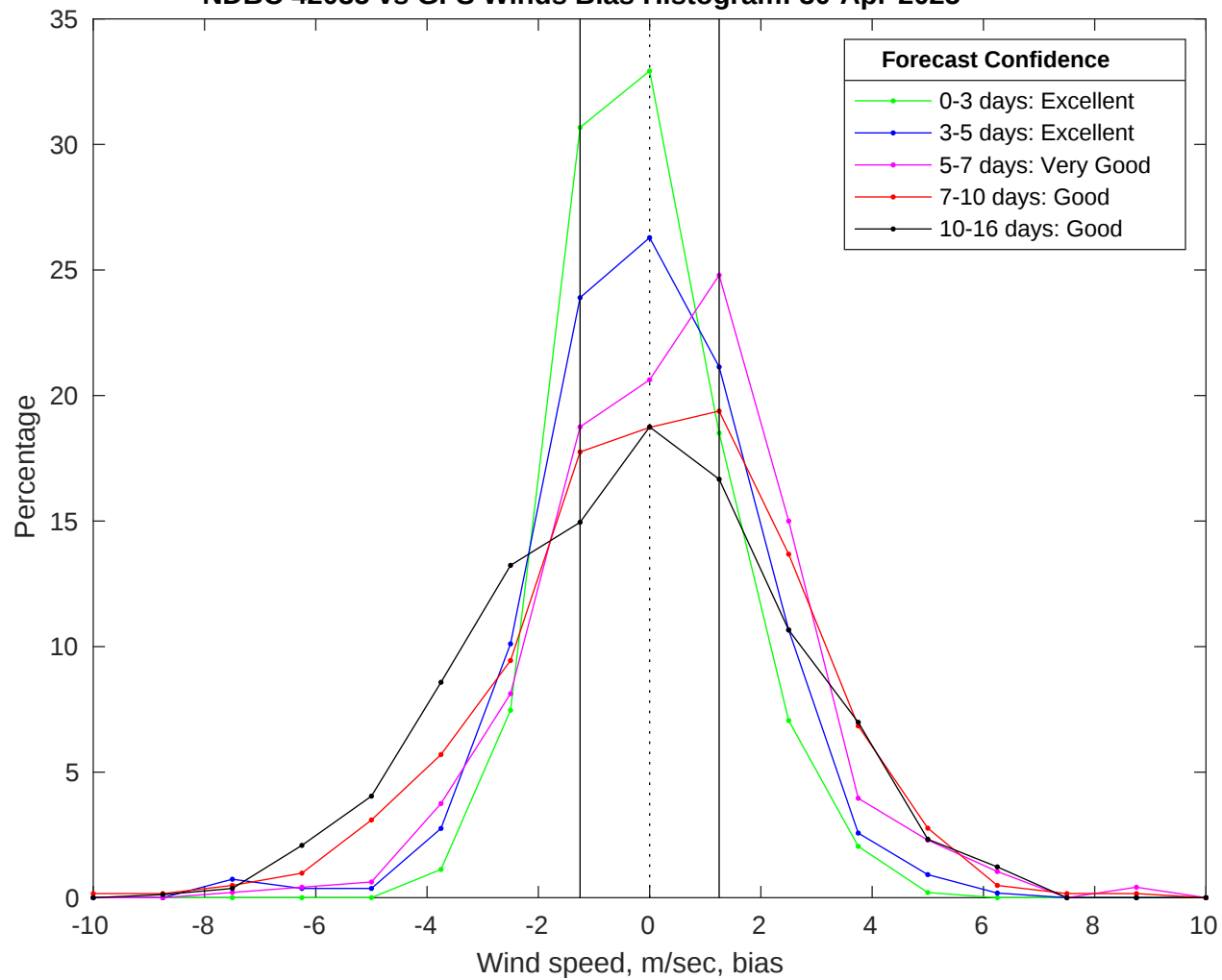
NDBC 42035 vs GFS Winds Bias Histogram: 30-Apr-2025
