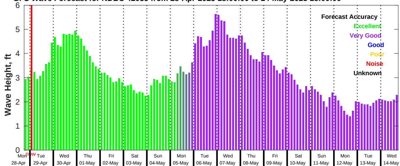
GFS Wave Forecast for NDBC 42035 from 28-Apr-2025 18:00:00 to 14-May-2025 18:00:00
