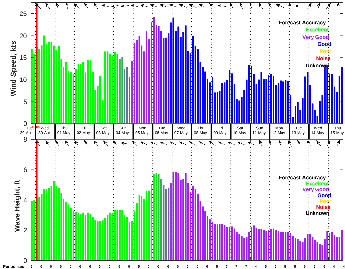
Wind & Wave Forecast for NDBC 42035 from 29-Apr-2025 18:00:00 to 15-May-2025 18:00:00
