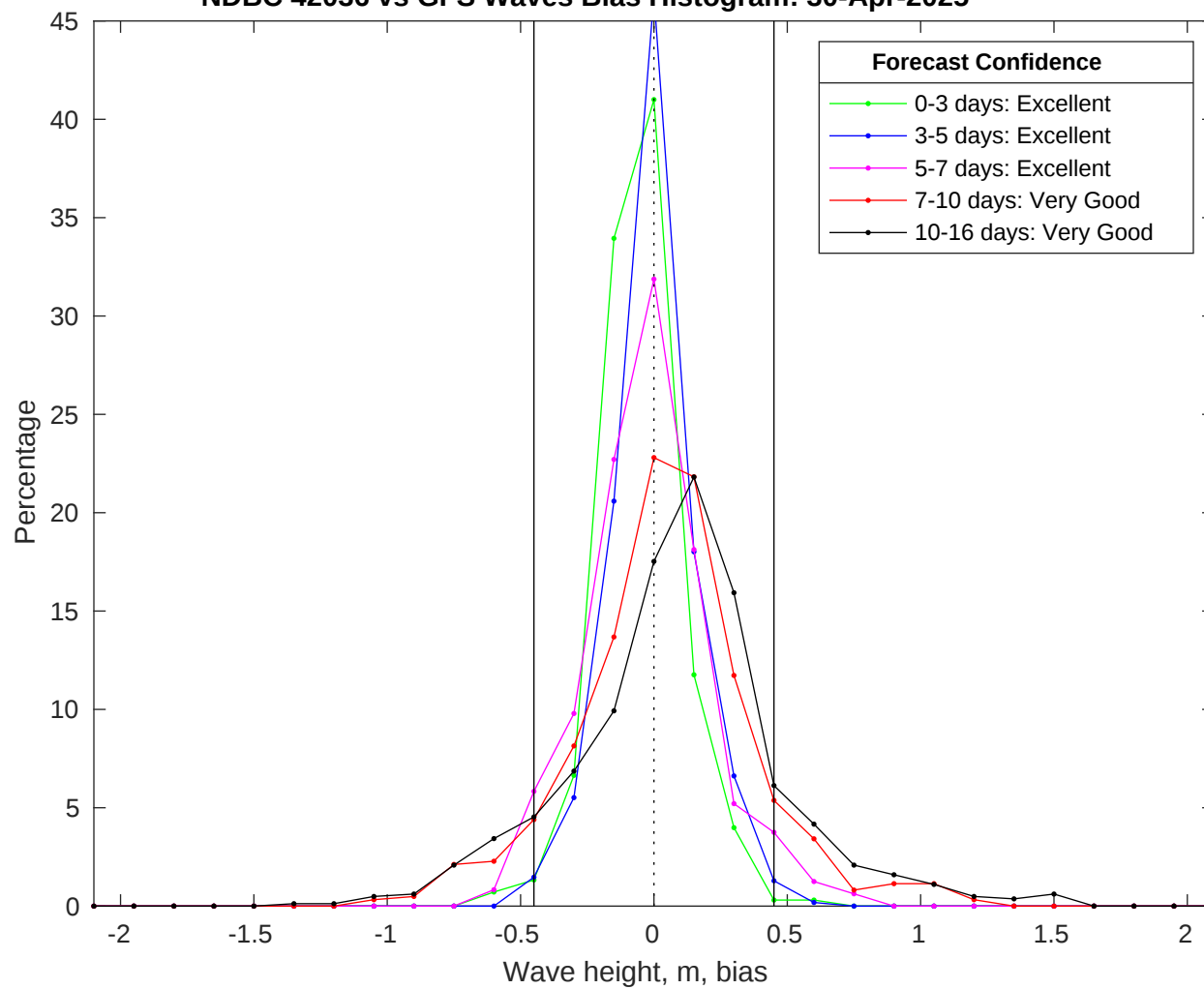
NDBC 42036 vs GFS Waves Bias Histogram: 30-Apr-2025
